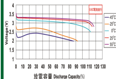
不同環境溫度下LYP類電池的放電特性曲線 Discharge characteristic curve of LYP type battery under different ambient temperature
