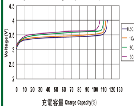
常溫下LYP類電池的充電特性曲線 Charge characteristic curve of LYP type battery under normal temperature
