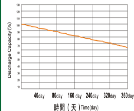
在常溫下LYP類電池的存儲特性曲線 Storage characteristic curve of LYP type battery under normal temperature
