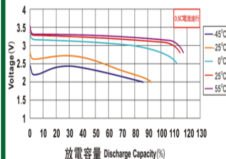
不同環境溫度下LYP類電池的放電特性曲線 Discharge characteristic curve of LYP type battery under different ambient temperature
