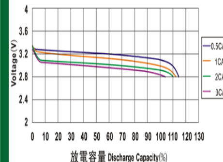
常溫下LYP類電池的放電特性曲線 Discharge characteristic curve of LYP type battery under normal temperature
