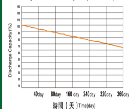
在常溫下LYP類電池的存儲特性曲線 Storage characteristic curve of LYP type battery under normal temperature
