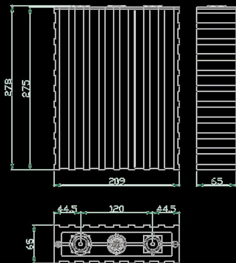
型号(MODEL): WB-LYP160AHA
