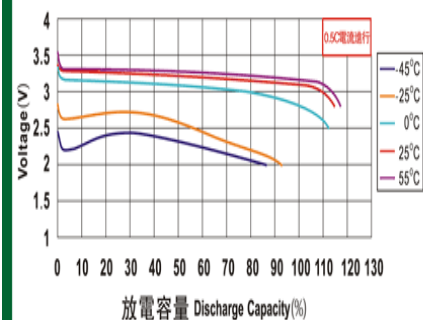
不同環境溫度下LYP類電池的放電特性曲線 Discharge characteristic curve of LYP type battery under different ambient temperature
