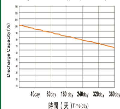
在常溫下LYP類電池的存儲特性曲線 Storage characteristic curve of LYP type battery under normal temperature
