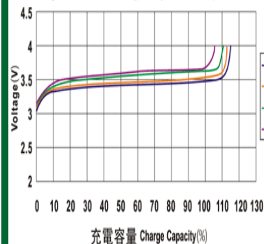
常溫下LYP類電池的充電特性曲線 Charge characteristic curve of LYP type battery under normal temperature
