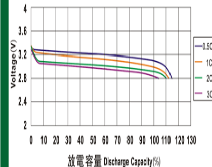
常溫下LYP類電池的放電特性曲線 Discharge characteristic curve of LYP type battery under normal temperature
