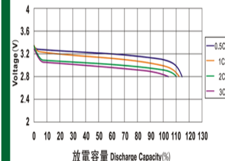
常溫下LYP類電池的放電特性曲線 Discharge characteristic curve of LYP type battery under normal temperature
