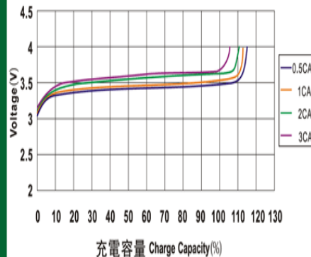
常溫下LYP類電池的充電特性曲線 Charge characteristic curve of LYP type battery under normal temperature
