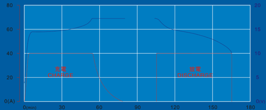
▲ WB-LP12V40AH在25℃環境下40A充放電特性 WB-LP12V40AH CHARGE AND DISCHARGE BY 40A AT TEMPERATURE OF 25°C
